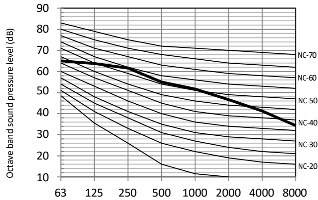
Figure 2-10.4: BCHC050N0A7-DTM140 octave band level
