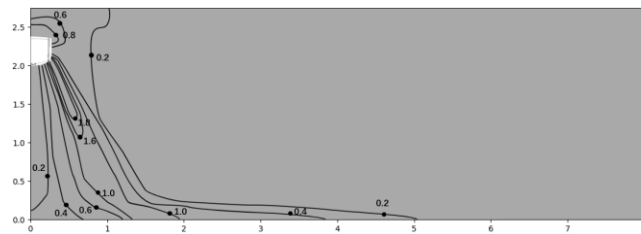
Figure 9.14: VEWM024T0A-DWV071 heating at 300S
