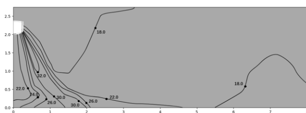
Figure 9.30: VEWM024T0A-DWV071 heating at 300S
