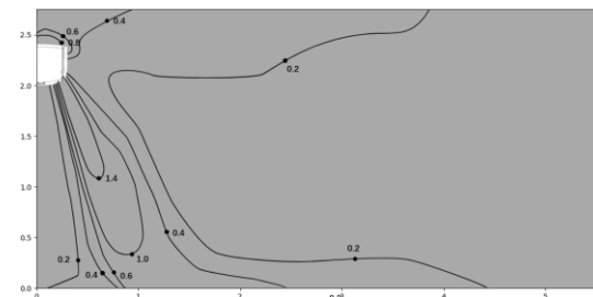
Figure 9.10: VEWM015T0A-DWV045 heating at 300S
