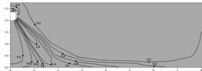
Figure 9.15: VEWM027T0A-DWV080 cooling at 300S
