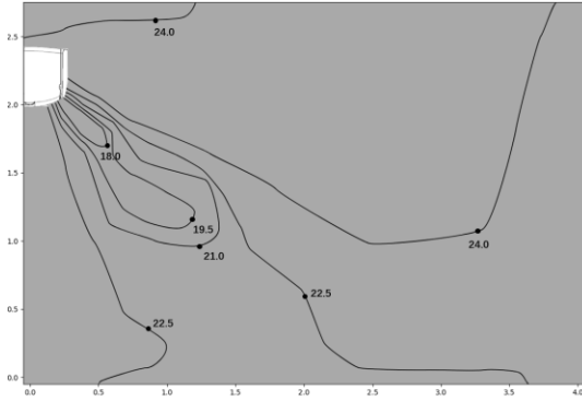
Figure 9.19: VEWM008T0A-DWV022 cooling at 300S
