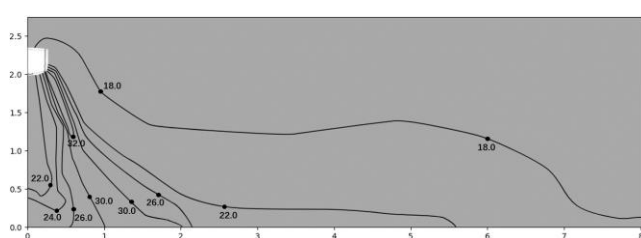
Figure 9.30: VEWM024T0A-DWV071 heating at 300S
