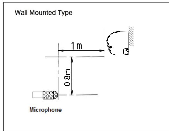
Figure 8.1: VEWM006(008,010,012,015,019,24,27) Wall mounted sound pressure level measurement
