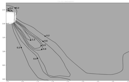
Figure 9.3: VEW008T0A-DWV022 cooling at 300S
