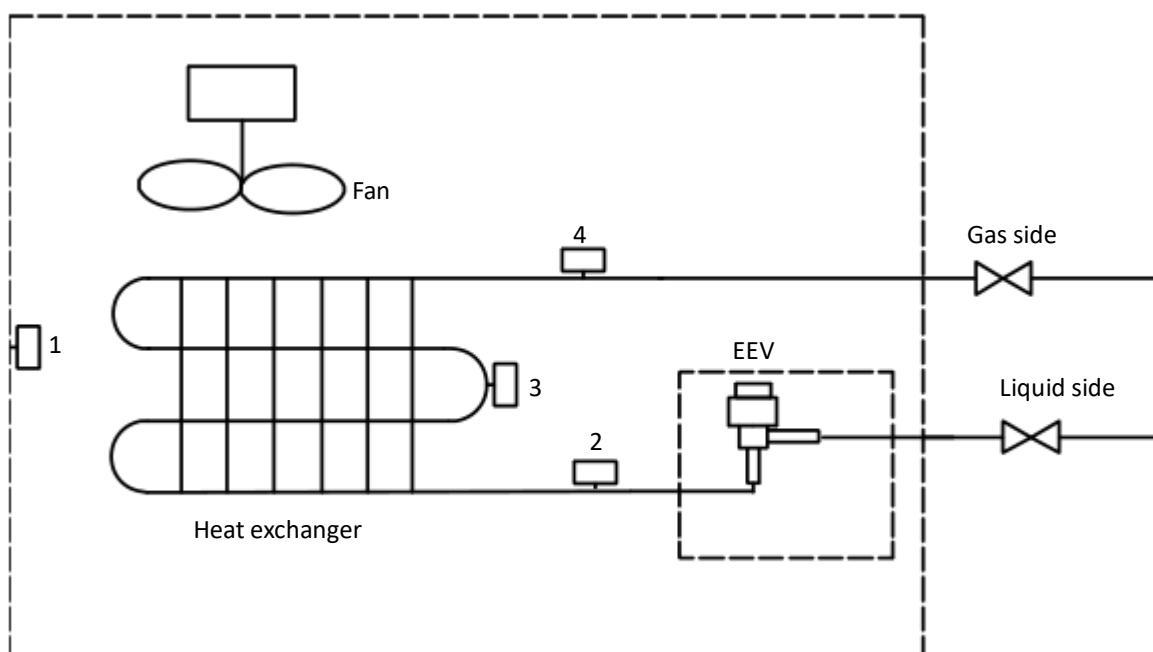
Figure 4.1: VEWM006(008,010,012,015,019,24,27) Wall mounted piping diagram
