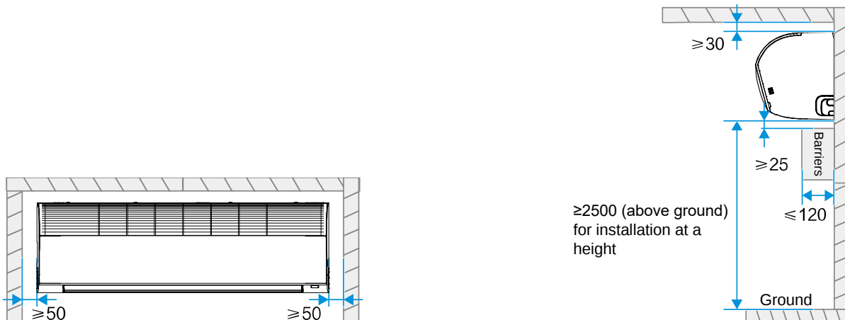
Figure 3.1: VEWM006(008,010,012,015,019) Wall mounted space requirements (unit: mm)
