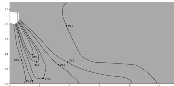
Figure 9.26: VEWM015T0A-DWV045 heating at 300S
