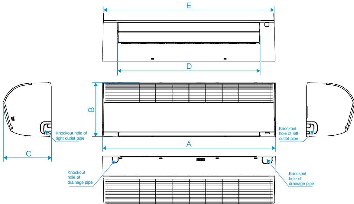
Figure 2.1: VEWM006(008,010,012,015,019,24,27) Wall mounted dimensions (unit: mm)
