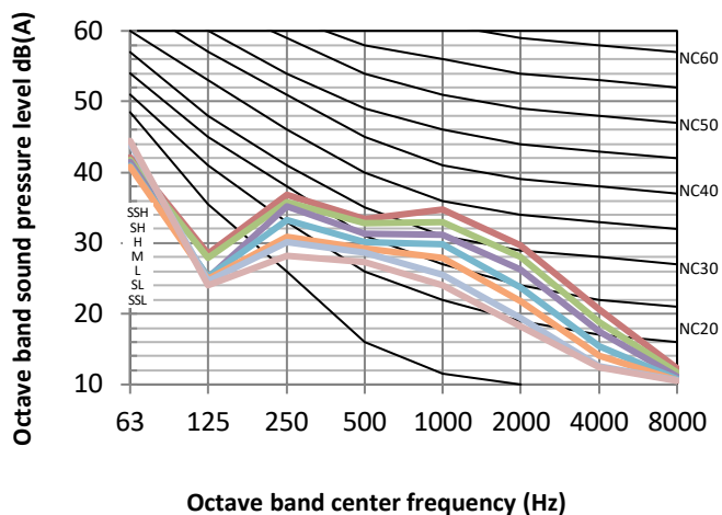
Figure 8.6: VEWM015T0A-DWV045 octave band levels
