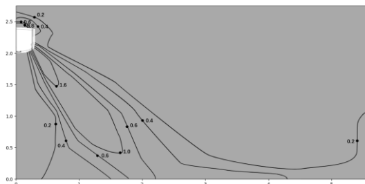
Figure 9.9: VEWM015T0A-DWV045 cooling at 300S
