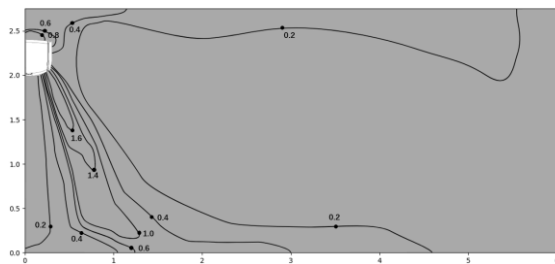
Figure 9.12: VEWM019T0A-DWV056 heating at 300S
