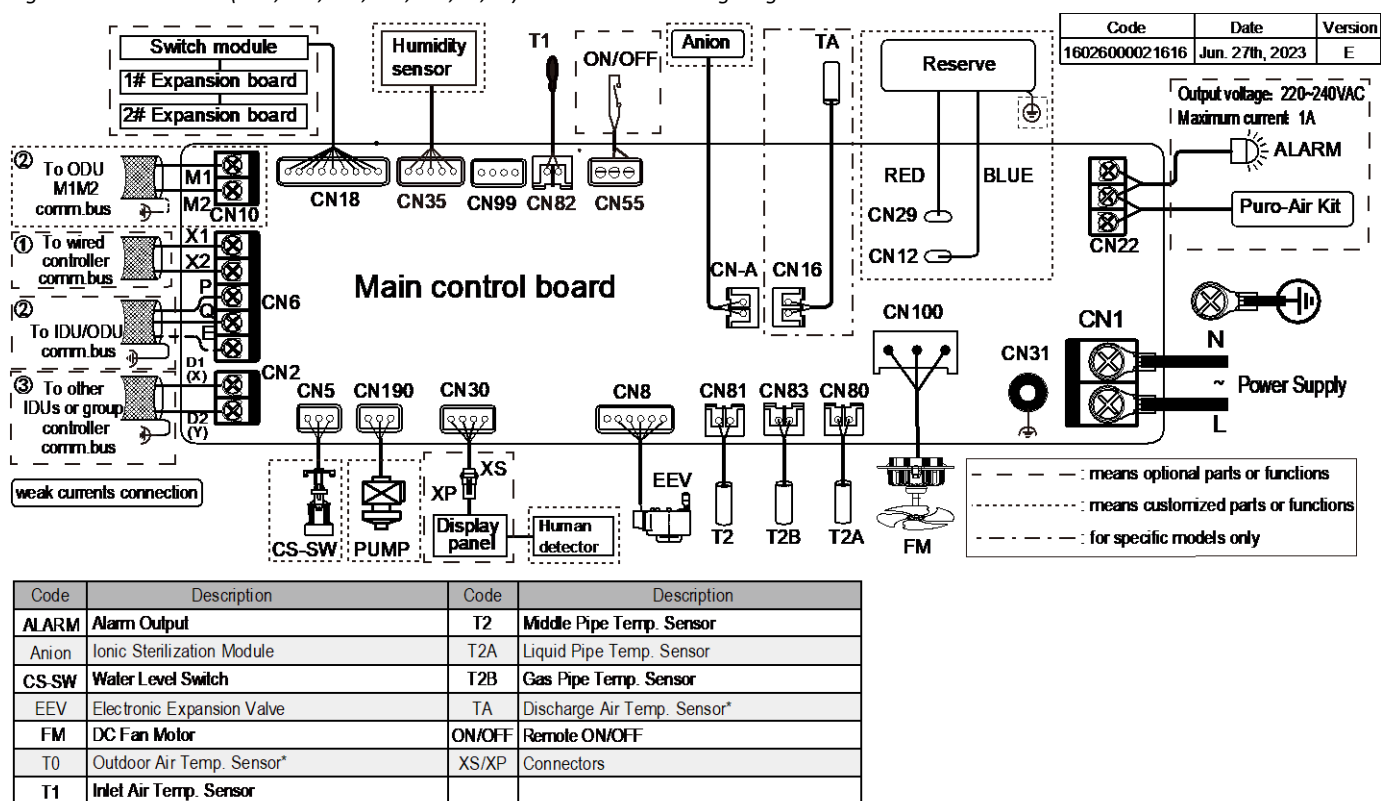
Figure 5.1: VEWMO06(008,010,012,015,019,24,27) Wall mounted wiring diagram
