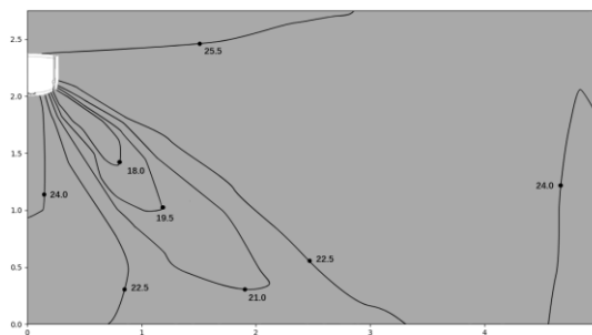
Figure 9.23: VEWM012T0A-DWV036 cooling at 300S
