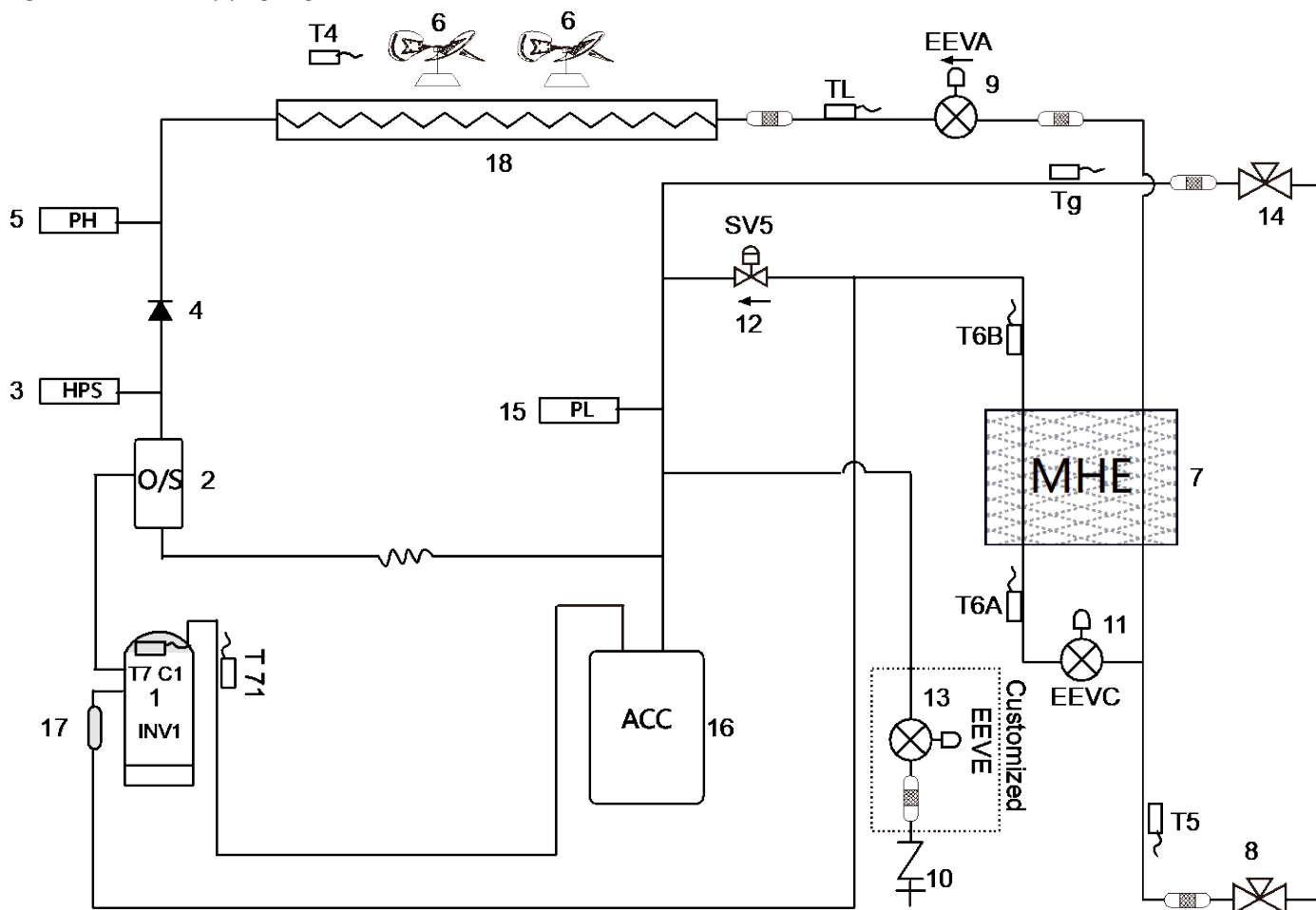
Figure 2-4.3: 22-24HP piping diagram
