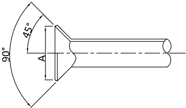
Figure 3-5.2: Flared opening
