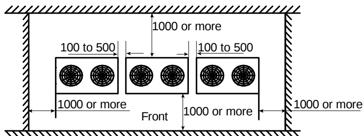
Figure 3-2.2: Single row installation (unit: mm)
