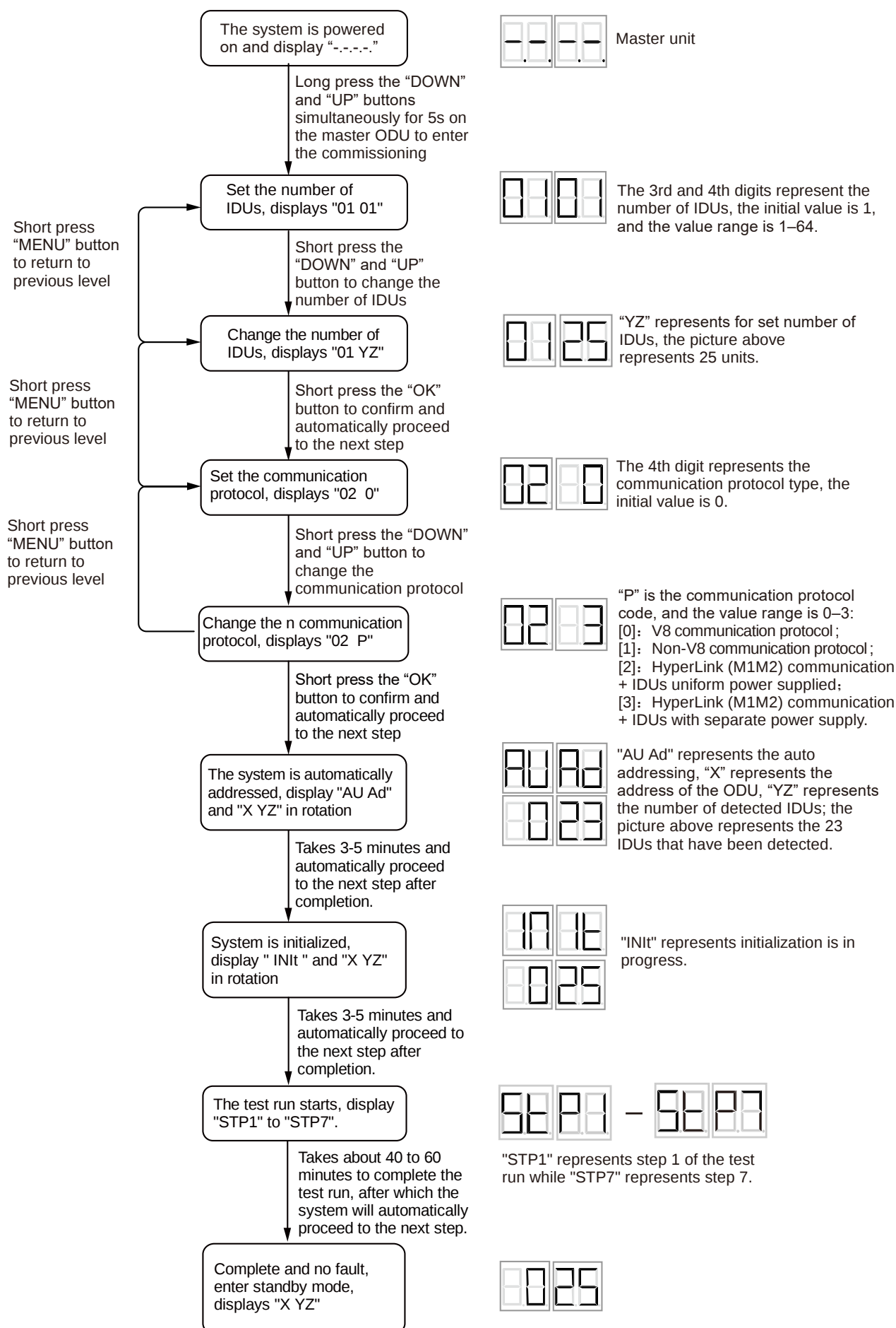
Figure 3-11.1: Commissioning Procedure
