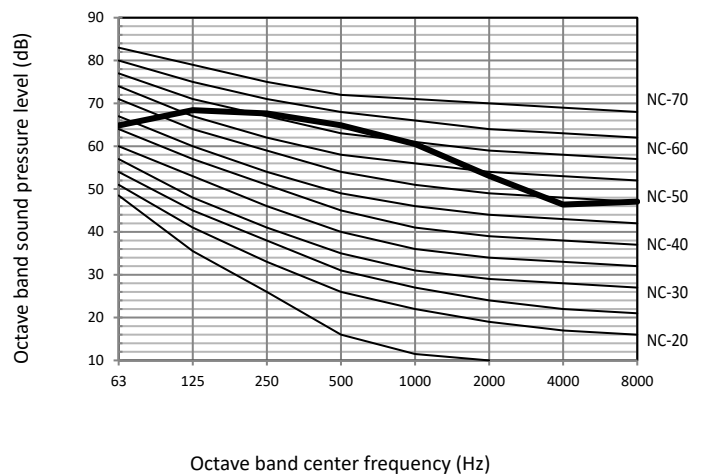
Figure 2-10.11: 26HP octave band level
