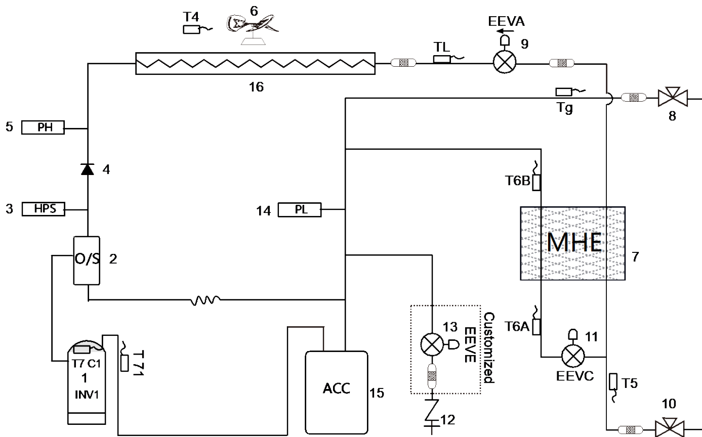
Figure 2-4.1: 8-12HP piping diagram
