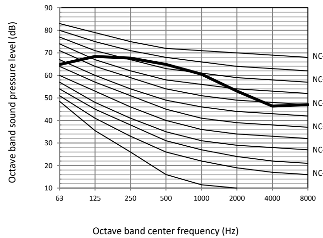
Figure 2-10.5: 14HP octave band level
