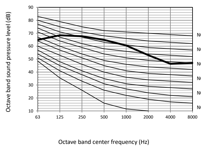
Figure 2-10.7: 18HP octave band level
