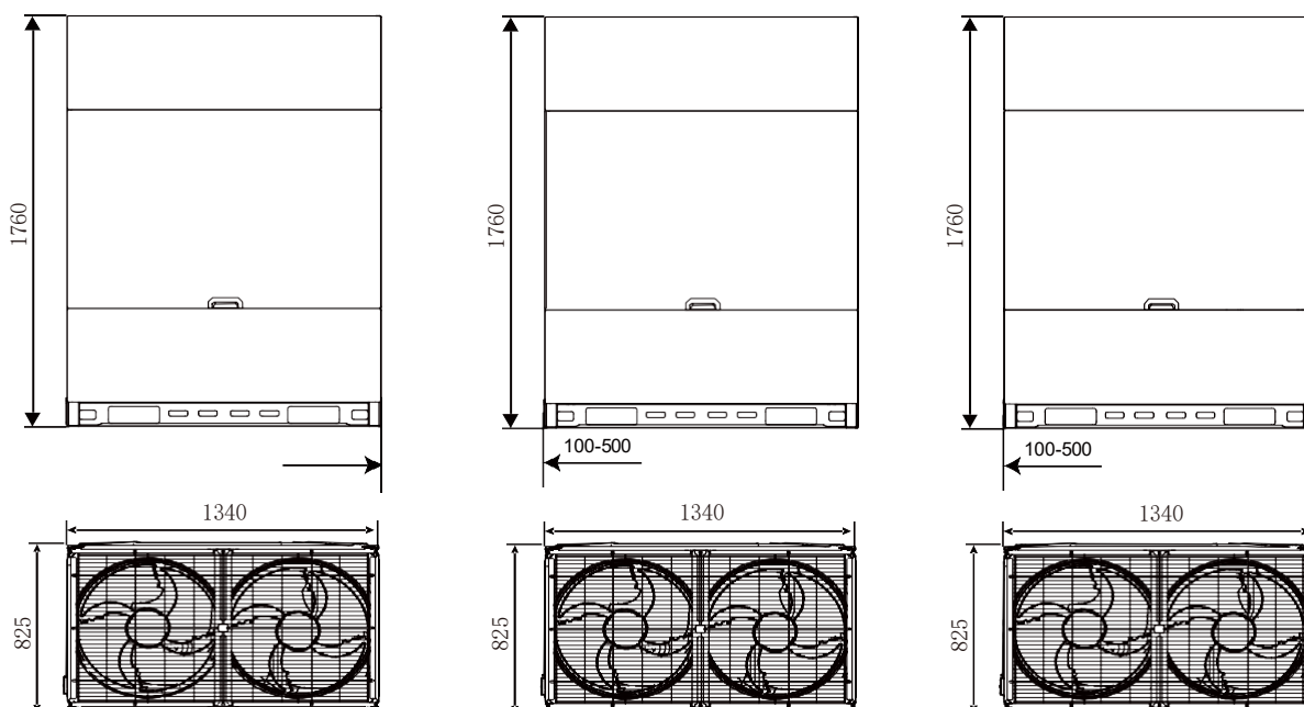
Figure 2-2.10: 82/84/86/88/90HP dimensions (unit: mm)
