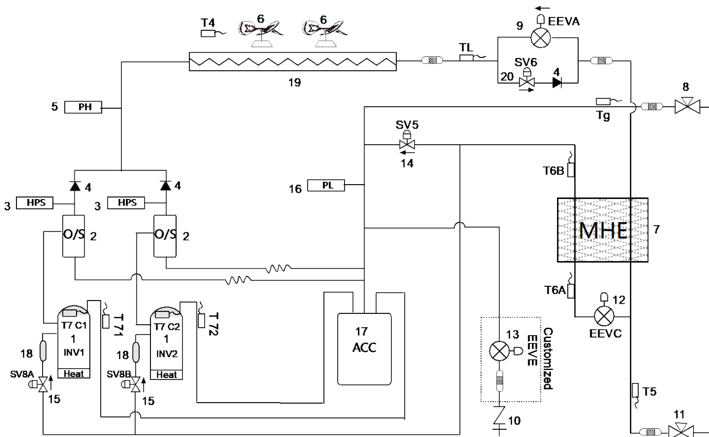
Figure 2-4.3: 26-30HP piping diagram
