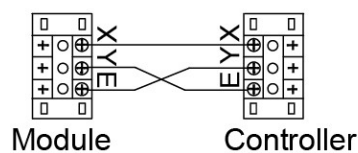
Incorrect connection
