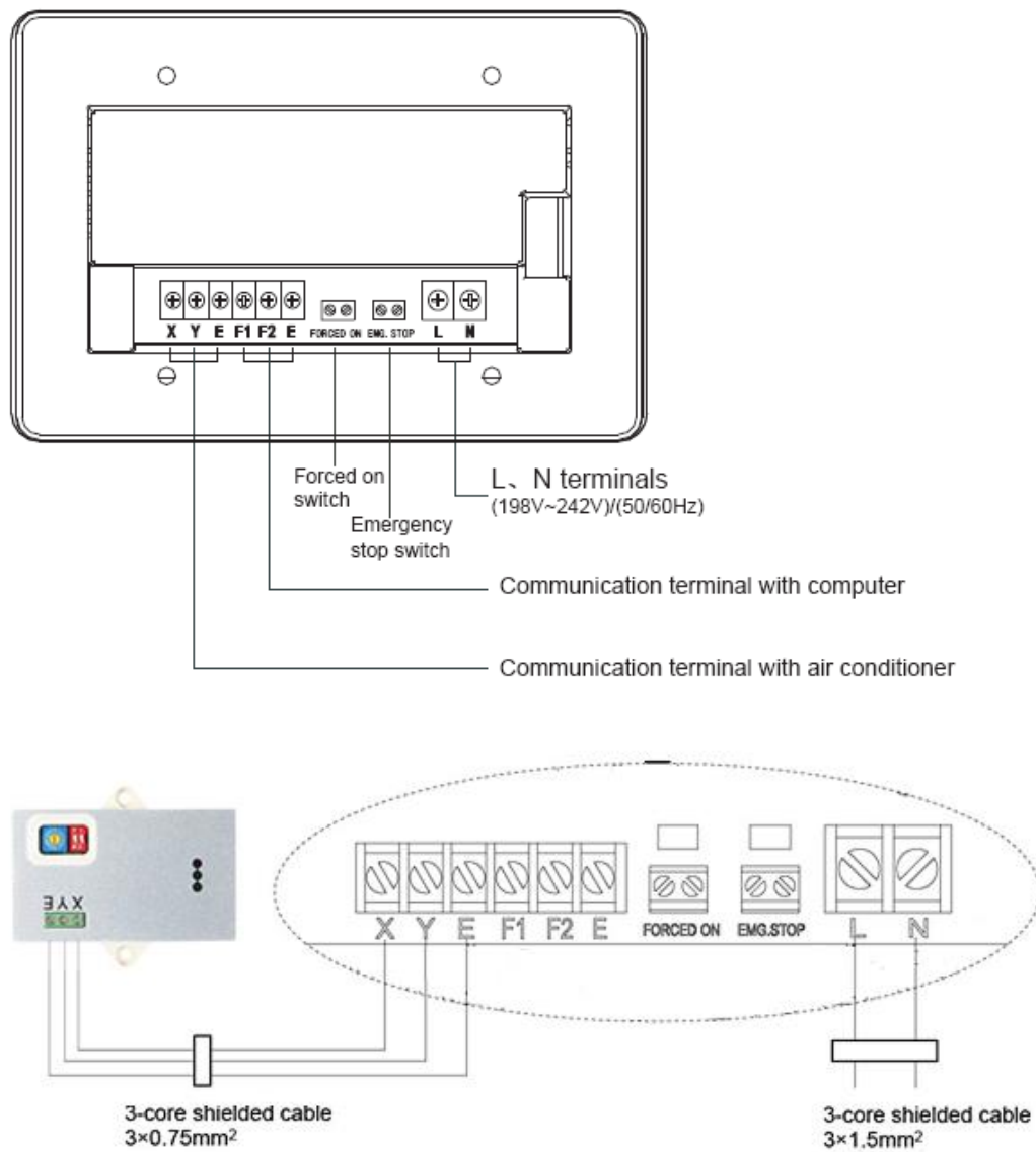
Correct connection
