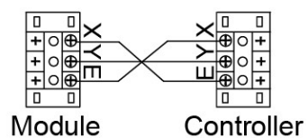
Incorrect connection
