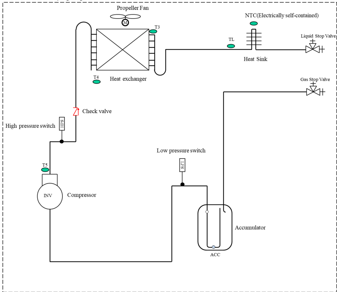
Figure 2-4.1: 28/36/42 model Piping diagram
