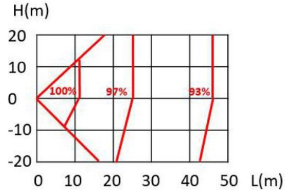
Figure 2-7.2: 42 model rate of change in cooling capacity
