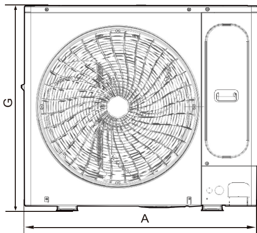
Figure 2-2.3: Model 48/56/60 Front view dimensions
