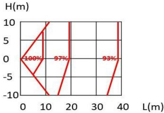
Figure 2-7.3: 48/56/60 model rate of change in cooling capacity
