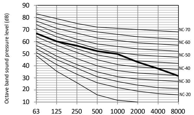
Figure 2-10.3: BCHC040N0A6-DTM115 octave band level
