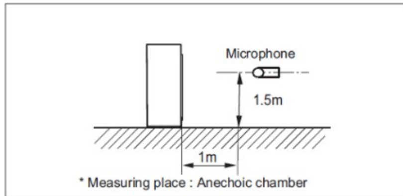
Figure 2-9.1: Sound pressure level measurement (unit: m)
