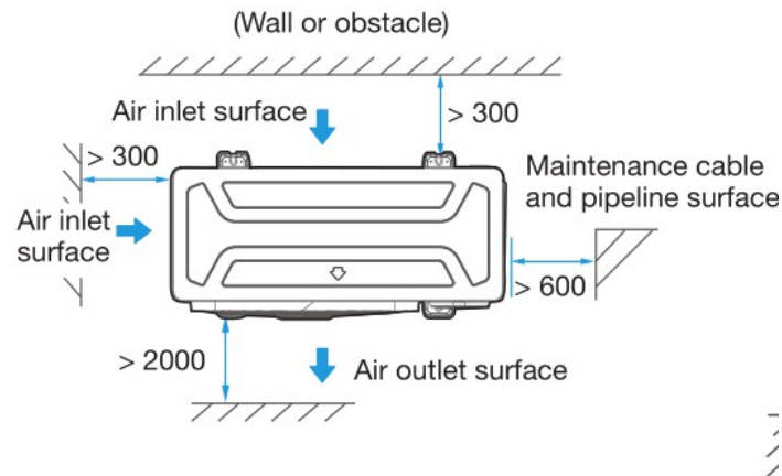
Figure 2-3.1: Single unit installation top view (unit: mm)
