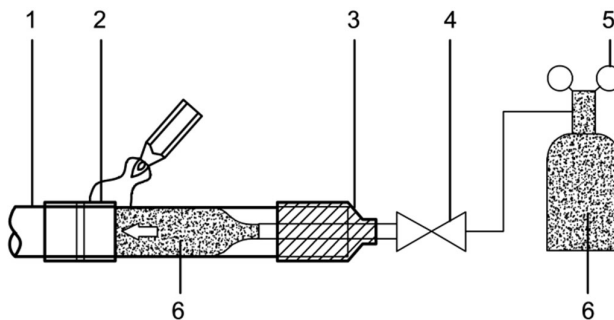
Figure 3-4.4: Flowing nitrogen through piping during brazing
