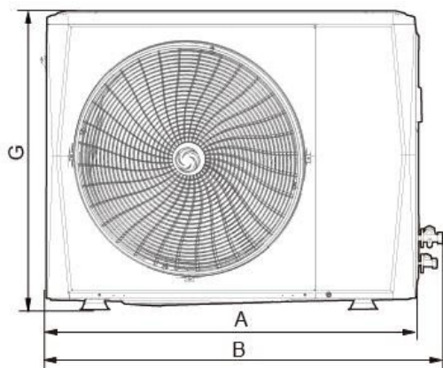
Figure 2-2.3: Model 48/56/60 Front view dimensions
