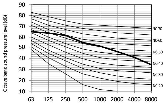
Figure 2-10.4: BCHC050N0A7-DTM140 octave band level
