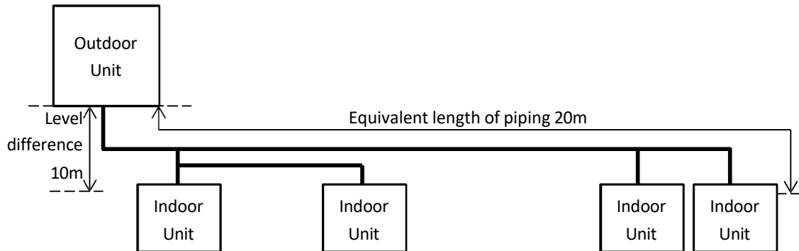
Figure 1-5.2: System diagram
