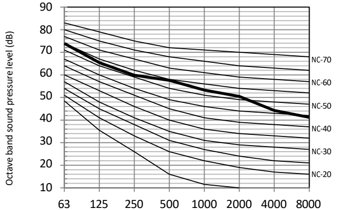
Figure 2-10.7: BCHC080N0A9-DTM200 octave band level
