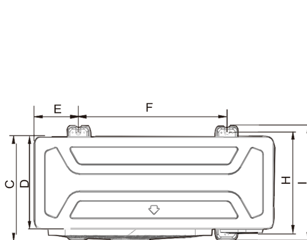
Figure 2-2.4: Model 48/56/60 Top view dimensions
