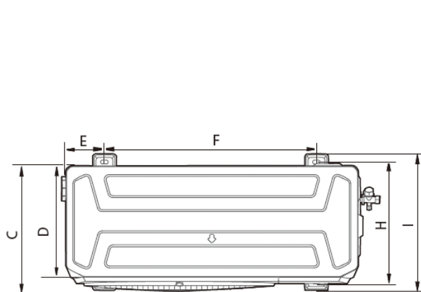
Figure 2-2.4: Model 48/56/60 Top view dimensions
