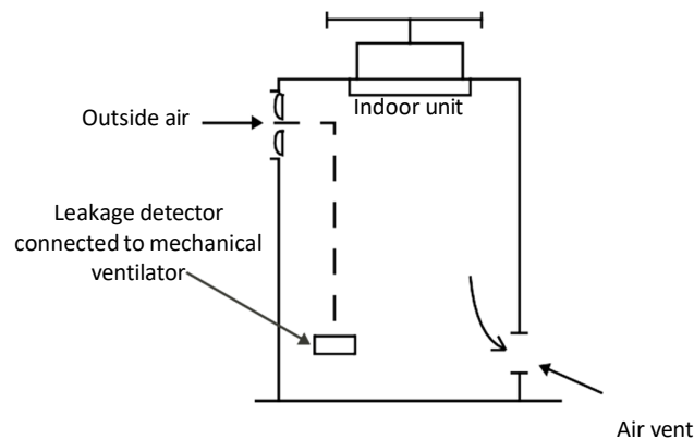
Figure 3-3.8: Mechanical ventilator controlled by refrigerant leak detector
