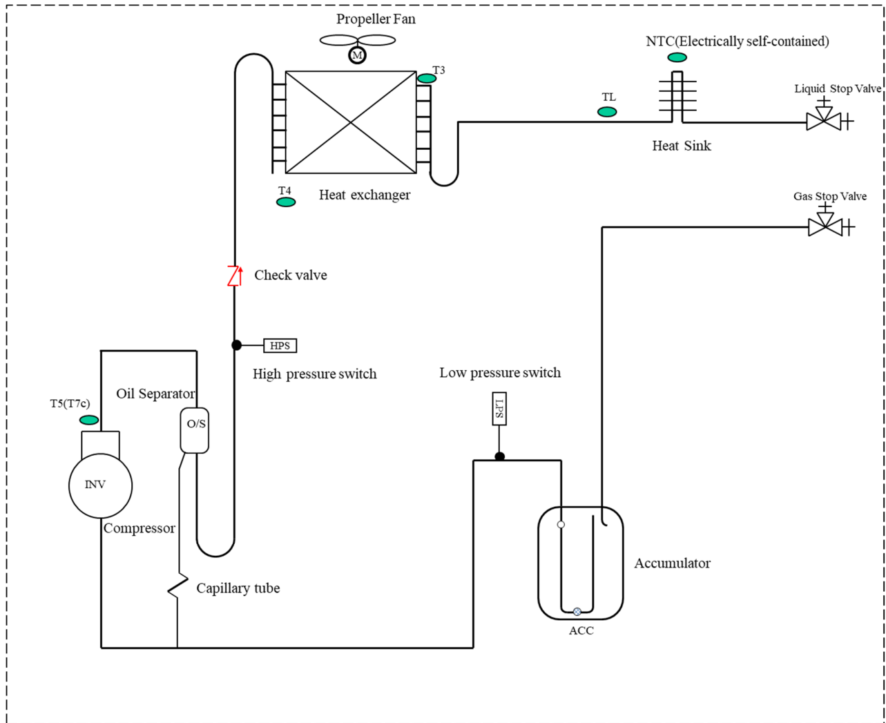
Figure 2-4.2: 48/56/60 model Piping diagram
