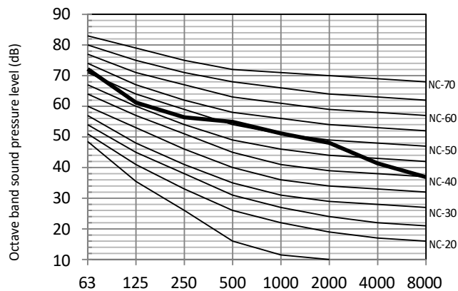
Figure 2-10.6: BCHC070N0A9-DTM190 octave band level
