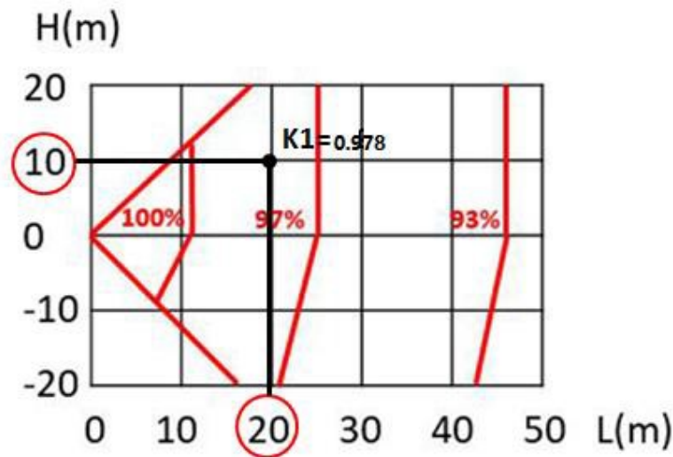
Figure 1-5.3: Ultima rate of change in cooling capacity
