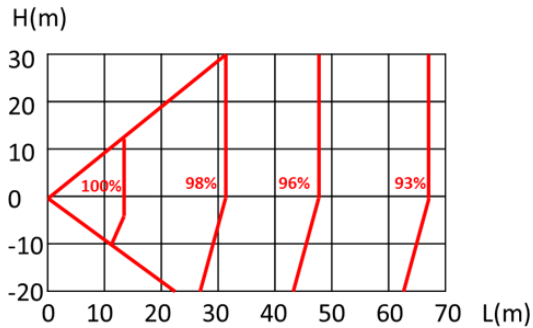
Figure 2-7.3: 48/56/60 model rate of change in cooling capacity
