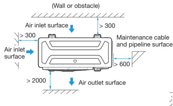
Figure 3-2.1: Single unit installation (unit: mm)
