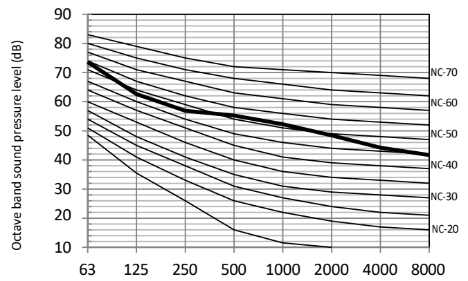
Figure 2-10.5: BCHC060N0A8-DTM160 octave band level
