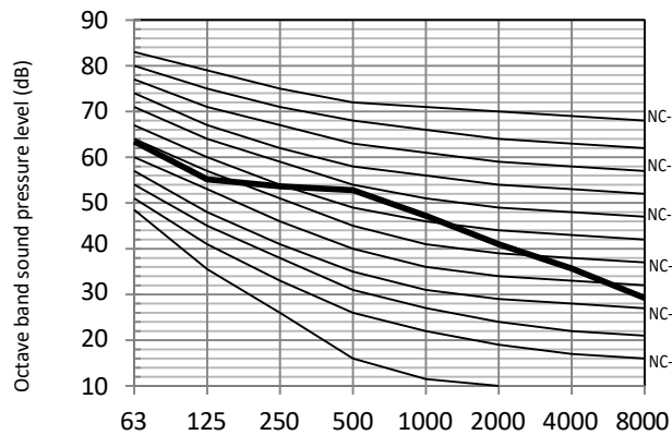
Figure 2-10.2: BCHC030N0A4-DTM090 octave band level
